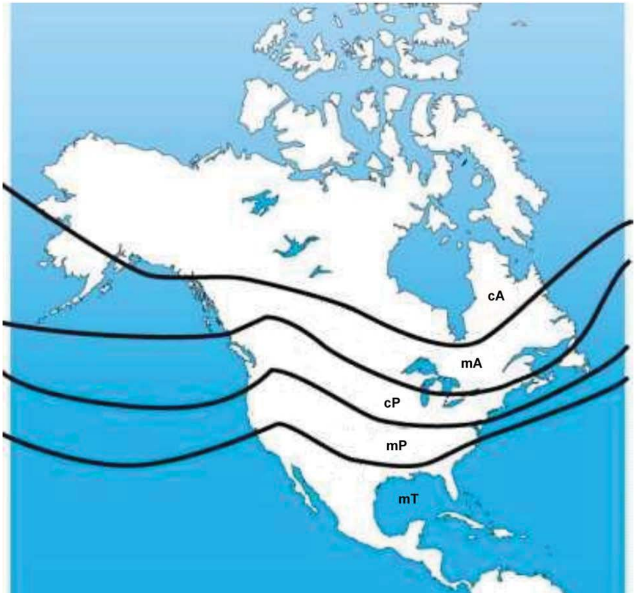
Figure 13L-1 North American Air Masses
