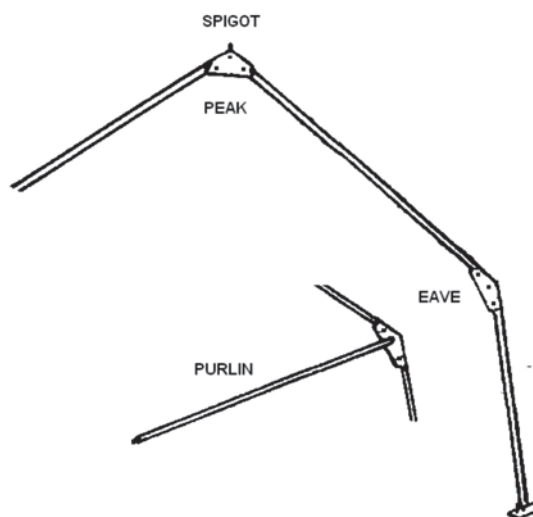
Figure 1 Frame
