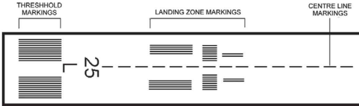
Figure 2 Runway Markings
